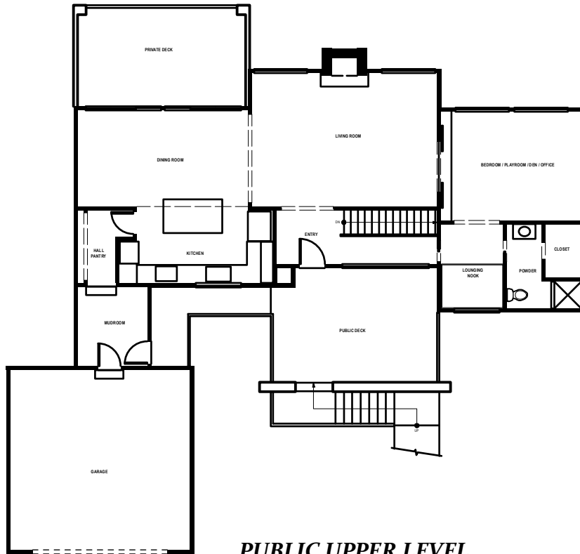
PUBLIC UPPER LEVEL 1,510 sf + garage
